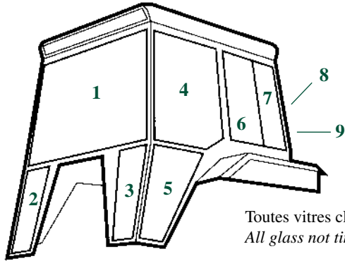
21/4002-2 (D7040, 04316689) Pare-brise Windscreen
