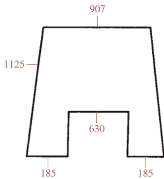
23/4000-84 (D9035, 5136368) Pare-brise Windscreen
